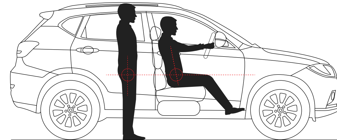
Hip-height ergonomic seat design for easy access
