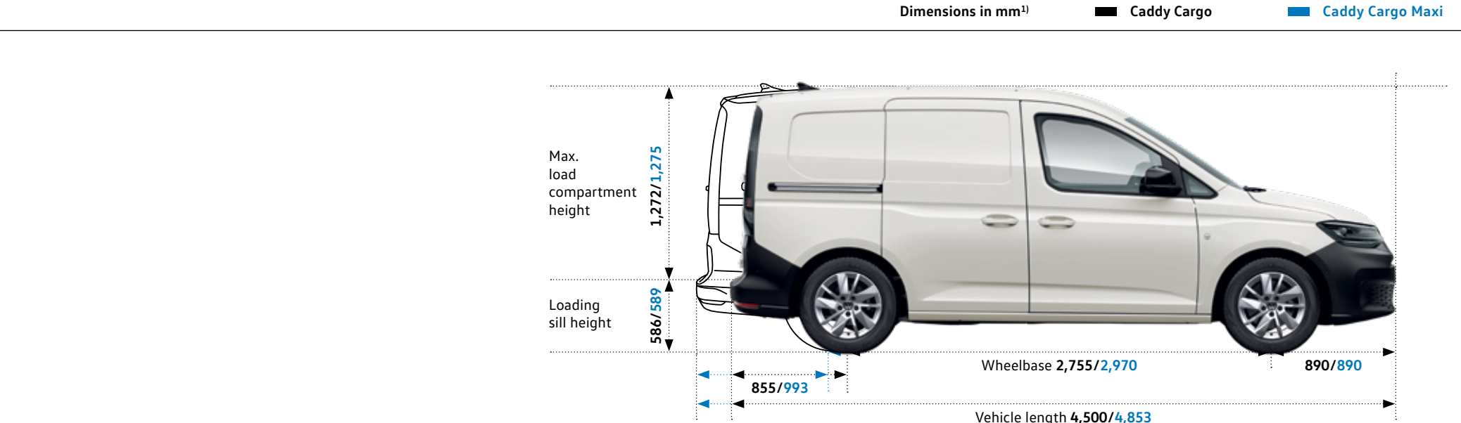
Load capacity in the Caddy Cargo panel van
