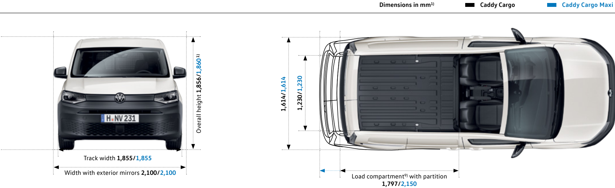
Wider Maxi sliding door (836 5) /846 x 1,095 mm) for Caddy Cargo Maxi 1)
