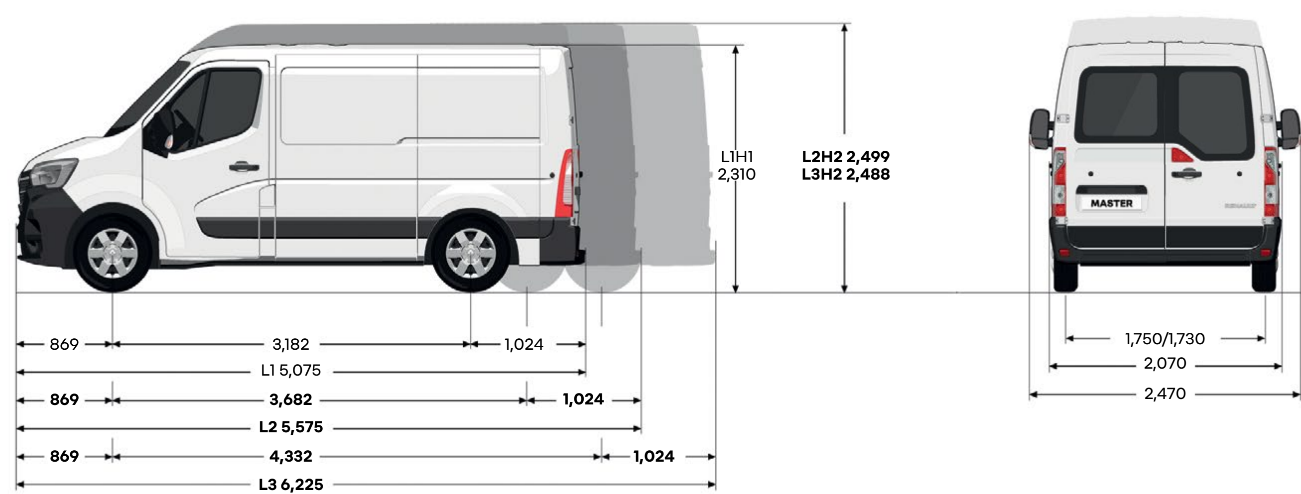
front-wheel drive panel van
