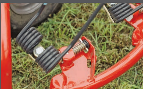
Tine position for raking: swept back. (Haybob 300 and 360)
