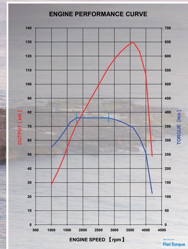
Isuzu 4JJ1-TC Hi-Power turbo diesel engine offers maximum torque output across a wide rev range minimising the need to change gears
