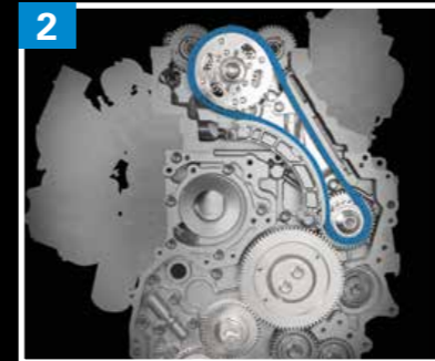
2 Steel timing chain (not poly belt)
