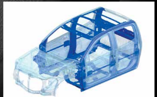
The cabin is constructed from high tensile tailor blank welded steel for unyielding strength and rigidity of the passenger safety cell
