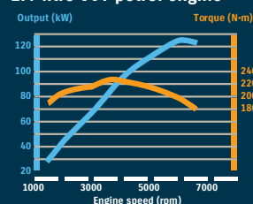
2.4-litre VVT petrol engine
