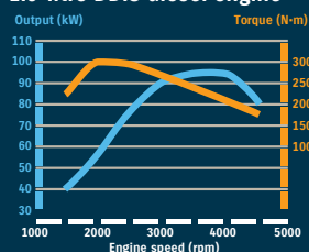
1.9-litre DDiS diesel engine
